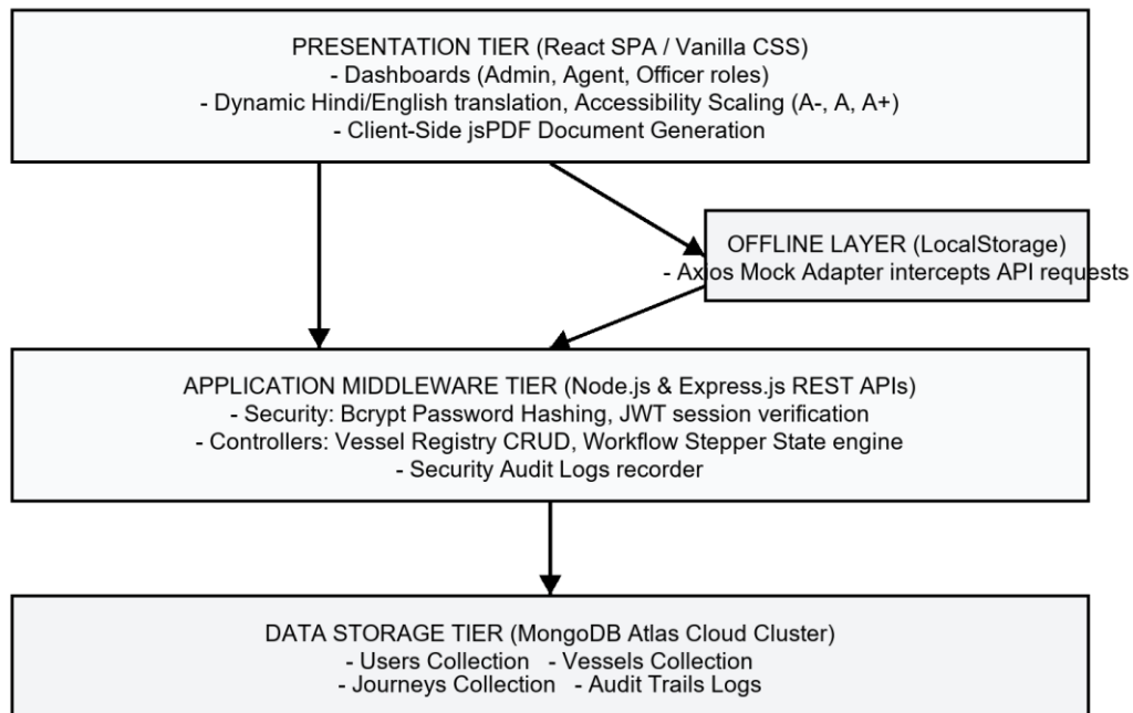
Figure 3.1: High-Level System Architecture Diagram
