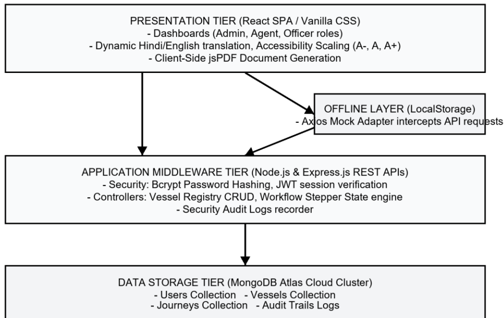
Figure 1.1: High-Level System Architecture Overview
